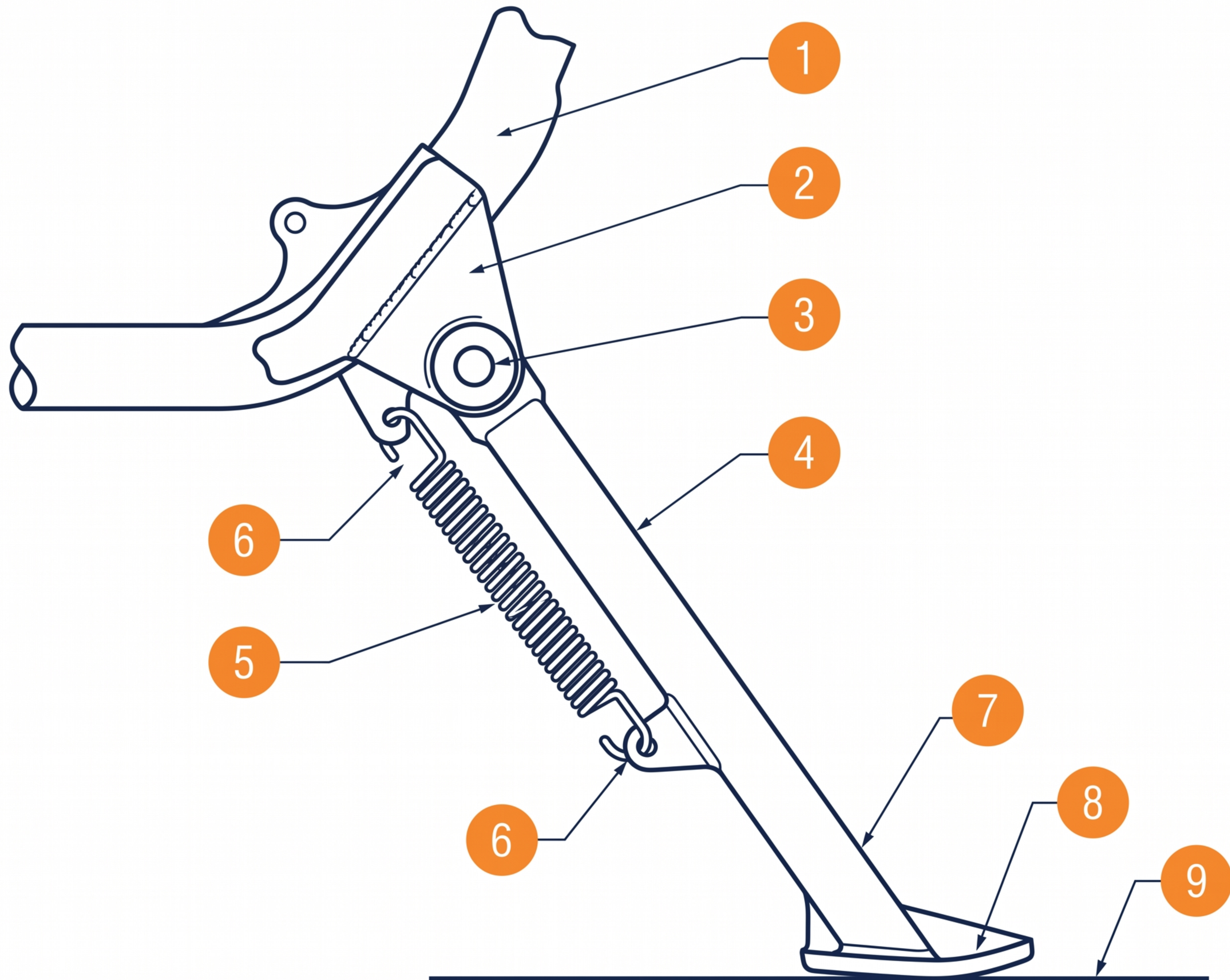
EA-02 Motorcycle Side Stand Assembly (Student Version)
